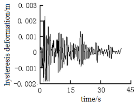
Figure 4: Response Curve Of Engineering Structure Hysteresis Deformation
