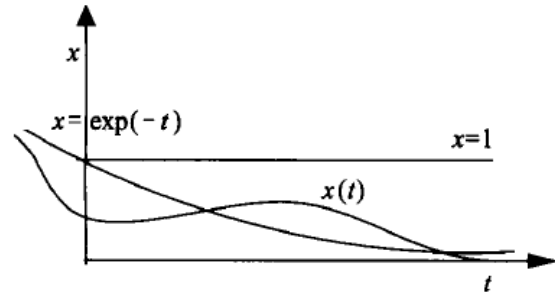
Figure 1: Schematic Diagram About The Stability Of Null Solution q Moment Expectation Index
