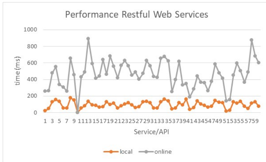
Figure 8. Processing Graph Service
