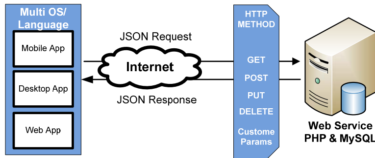
Figure 4: Software System Model
