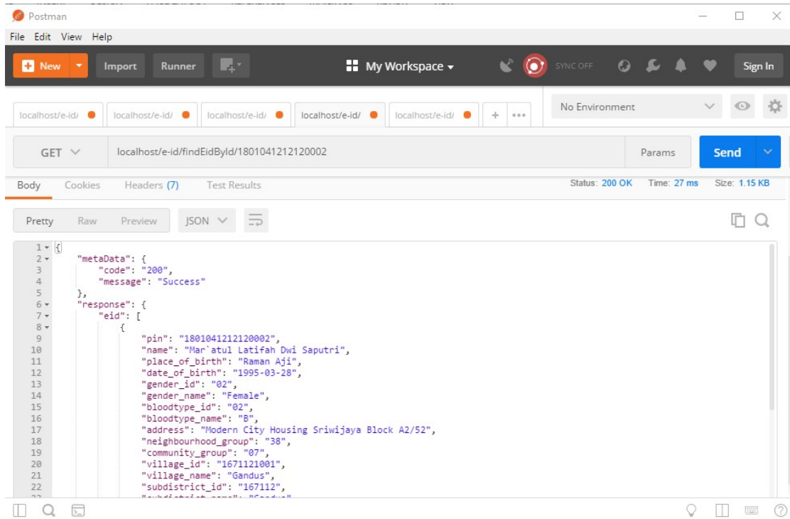
Figure 6: Testing using Postman Software
