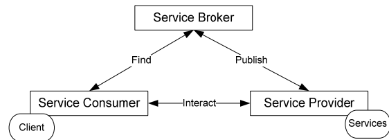
Figure 1: SOA Architecture
