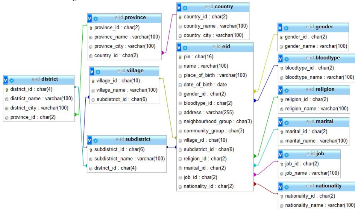
Figure 5: Physical Database Diagram
