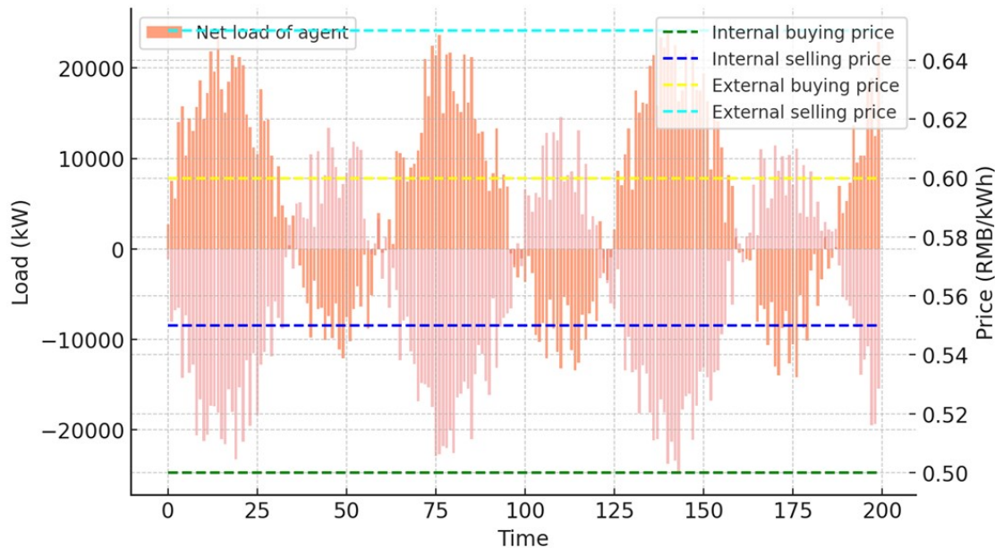
Figure 6: Load and internal price for different agent
